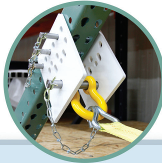
LOWER RACK CONNECTION
